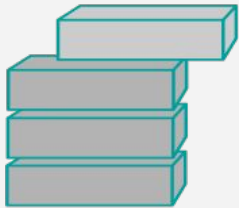
Product Backlog
